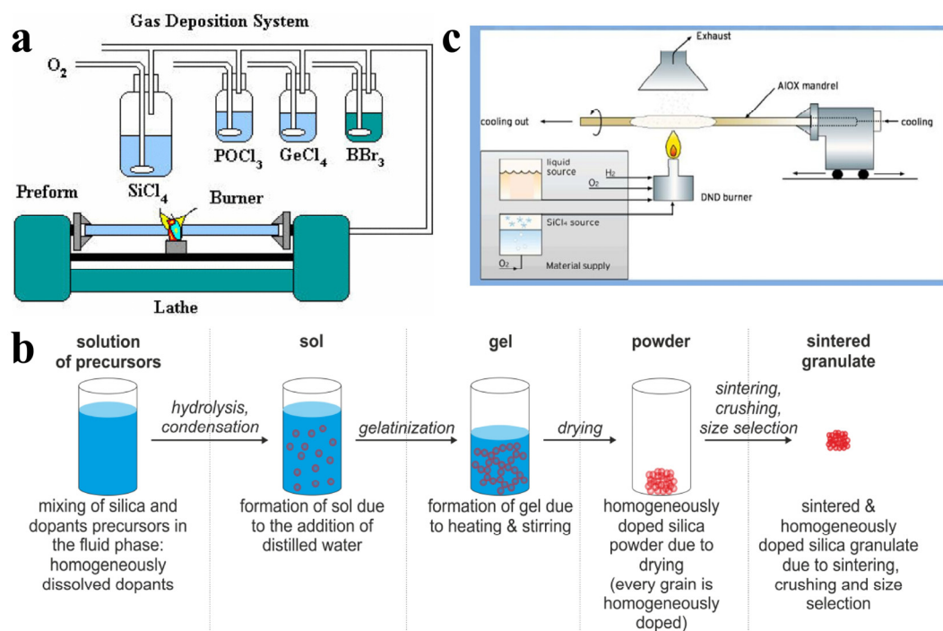
Figure 1. (a) Schematic diagram of an MCVD system [57]. 2020, IEEE Photonics Journa. (b) Basic principle of the sol-gel process [60]. 2017, Fibers. (c) Schematic of the direct nanoparticles deposition (DND) process [65]. 2017, Fibers.
