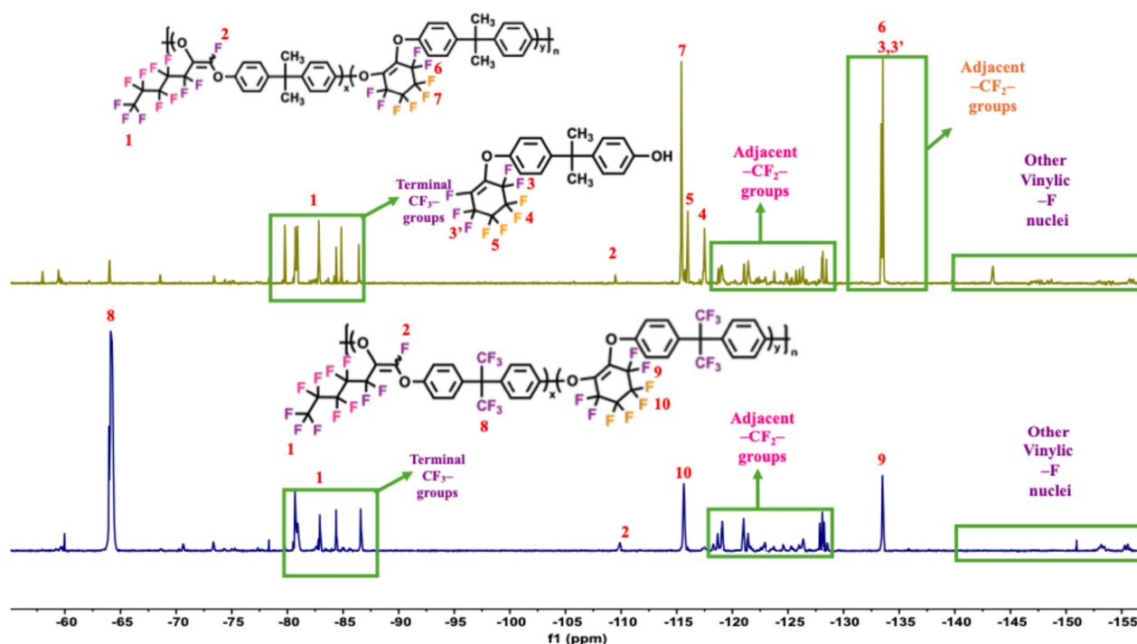
Figure 4. ^{19}\text{F} NMR (470 MHz, \text{CDCl}_3 ) analysis of copolymers poly(2-co-4)A (top), and poly(2-co-4)AF (bottom).
