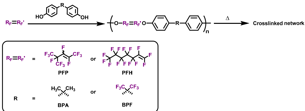
Figure 1. Previous study scheme featuring polymerization of acyclic perfluoroolefins with aromatic bisphenols [14].
