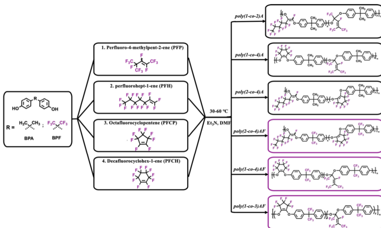
Figure 2. Step-growth copolymerization scheme of cyclic/acyclic perfluoroolefins with bisphenols.
