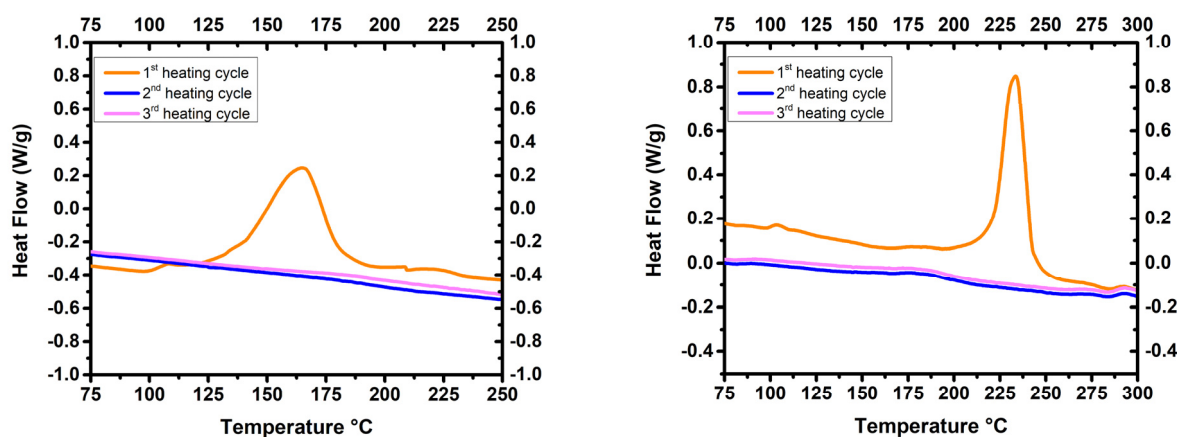
Figure 6. DSC analysis (10 °C/min in N 2 ) of poly(2-co-4)A (Left) and poly(2-co-4)AF (Right).
