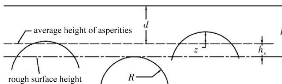
Figure 11. Asperity model of rough surface.
