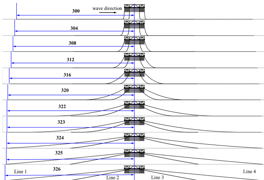
Figure 6. Mooring condition diagram.
