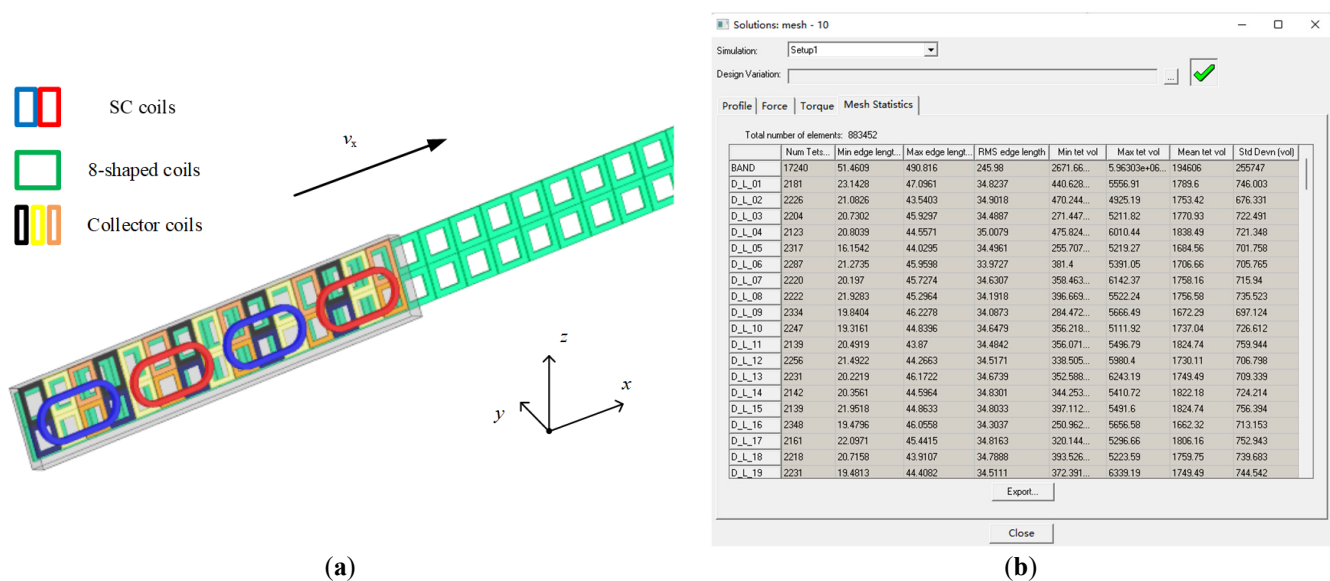
Figure 7. The finite element model at k = 3 of EDS maglev. (a) FEM; (b) mesh data.
