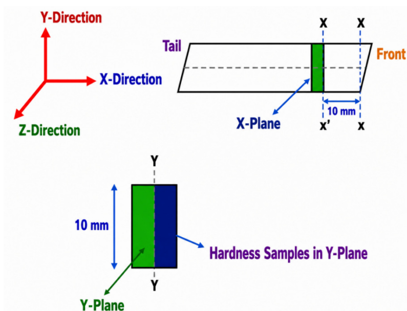
Figure 5. Cutting procedure of ECAPed samples.
