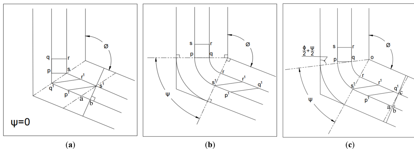
Figure 8. (a) Case (a) when ( \psi = 0^\circ ). (b) Case (b) when ( \psi = \pi - \phi ). (c) Case (c) when ( \psi ) lie between ( \psi = 0^\circ ) and ( \psi = \pi - \phi ).
