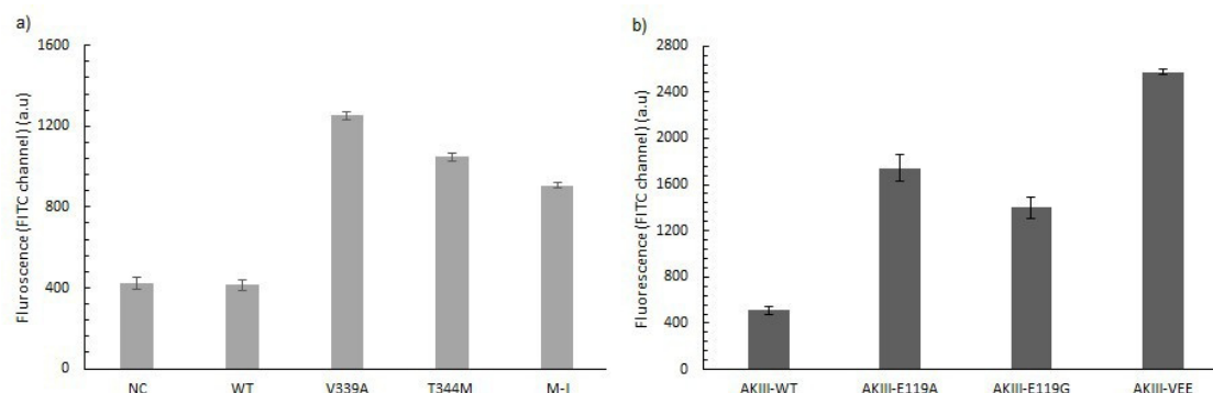
Figure 6. (a) Fluorescent emission of ATP sensor of wildtype AKIII in comparison with feedback resistant mutant AKIII produced in fully automated system at lysine concentration of 200 mM (error bars indicate 1% confidence interval n = 50000 ). (b) Fluorescent signal of wildtype AKIII in comparison with AKIII mutants with different substrate specificity (malate instead of aspartate) (same error bars).
