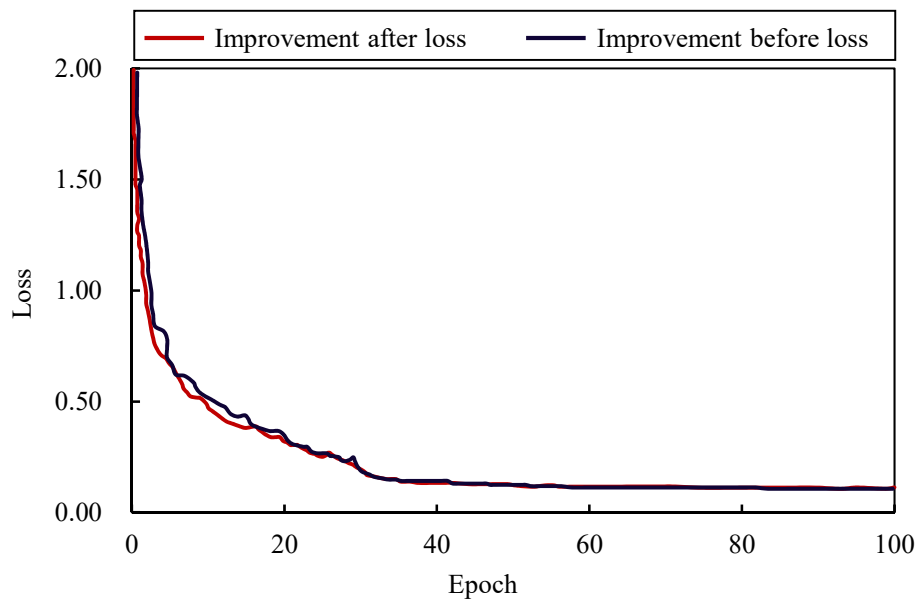
Figure 12. Training loss curves of the model before and after improvement over training epochs.
