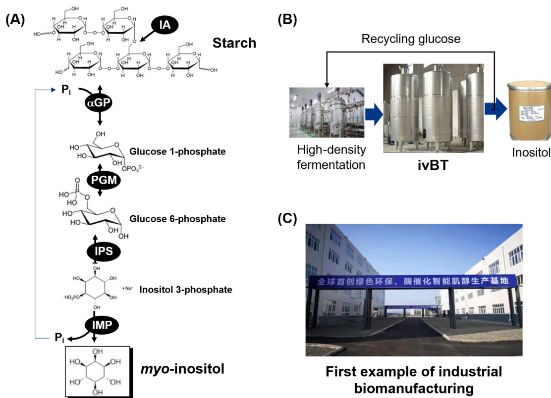
Figure 6. Schematic presentation of the in vitro starch-to-inositol pathway (A), wherein enzymes are αGP (α-glucan phosphorylase), PGM (phosphoglucomutase), (iii) IPS (inositol 3-phosphate synthase), (iv) IMP (inositol monophosphatase), and IA (isoamylase); the concept of two-step biomanufacturing as well as product separation and glucose reuse (B); and image of the first large-scale inositol factory (C).
