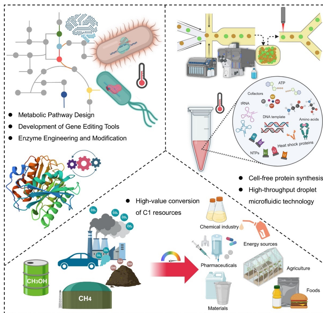
Figure 4. Perspectives of leveraging thermophiles and thermozymes as high-temperature catalysts.
