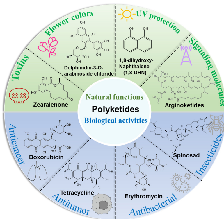
Figure 1. Diverse biological activities of polyketides. Delphinidin-3-O-arabinoxide chloride is a PKS-derived product, which is formed through further modifications by using the PKS-mediated synthesis of the key intermediate chalcone; 1,8-DHN is the immediate precursor of melanin synthesis, which synthesized by PKS utilizing acetyl-CoA or malonyl-CoA.
