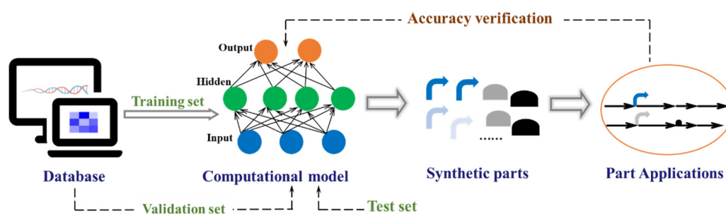
Figure 7. Artificial intelligence predicts biological parts. A portion of the existing sample databases is selected as the training set, and the computational model is selected to train the parameters, while the other portion of the sample databases is utilized as the validation set to refine and optimize the model parameters. After training is completed, the model is evaluated by using the test set. The model is then used to predict the biological parts that meet the requirements, and finally, the accuracy of the model is verified through actual experimental results.
