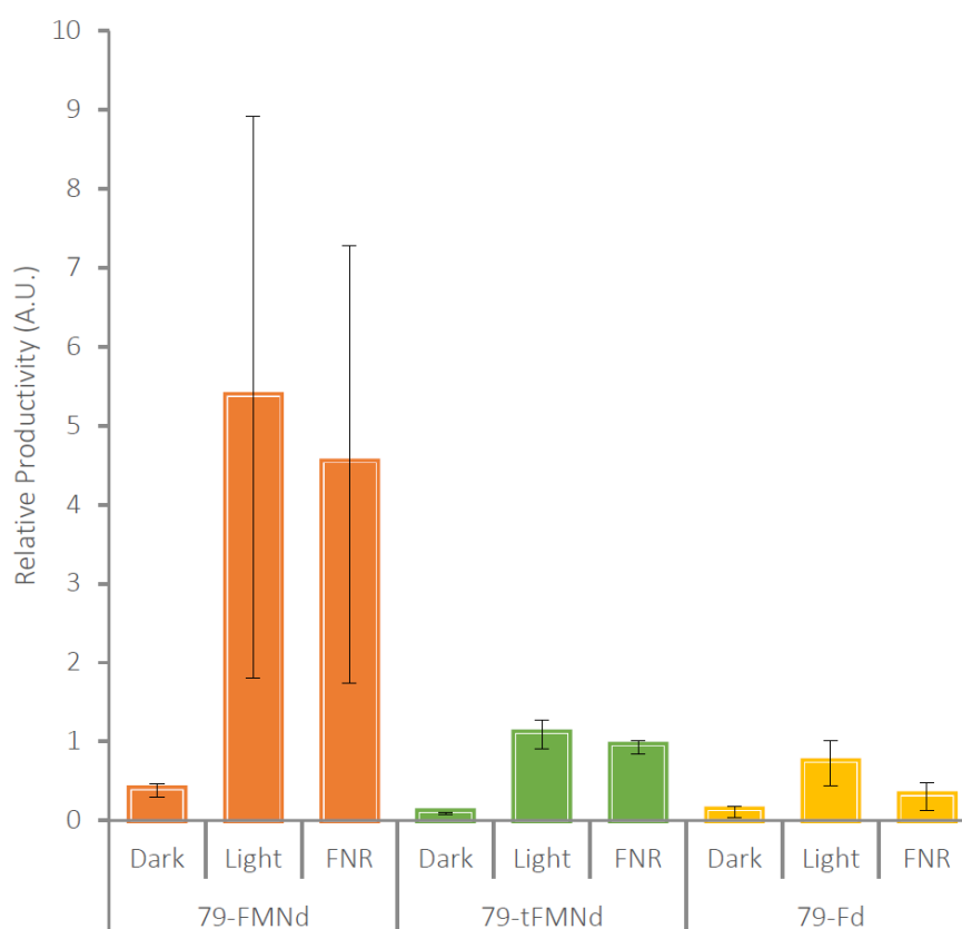
Figure 4. In vitro light driven assays. Thylakoids extracted from strains expressing fusion constructs were assayed p -hydroxyphenylacetaldoxime formation in the dark, light, and in the presence of the competing electron sink FNR and NADP + . p -hydroxyphenylacetaldoxime was normalized to relative protein abundance in the thylakoid membranes.
