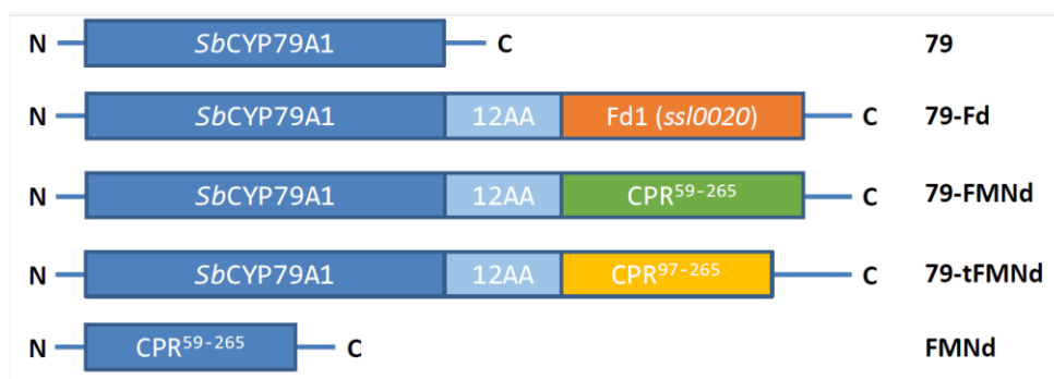
Figure 1. Constructs used in this study. Constructs depicted are located on a pDF- trc backbone under the IPTG inducible trc promoter. Construct abbreviations are given to the right of each construct. A pDF- trc backbone without any DNA insert is used as empty vector control.
