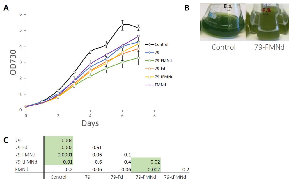
Figure 2. Growth characteristics of analysed strains. (A) Strains were grown photoautotrophically for seven days in triplicate and optical density was measured at 730 nm daily (OD 730 ). (B) Photo of the empty vector control to the left and 79-FMNd to the right. The empty control displays a color indicative of normal growth and the 79-FMNd strain displays a color indicative of chlorosis. (C) The resulting density on the last day was calculated for pairwise significance on the last day (Holms-Sidak). p -values are given in the table below the graph with significant pairs ( p < 0.05) highlighted in green.
