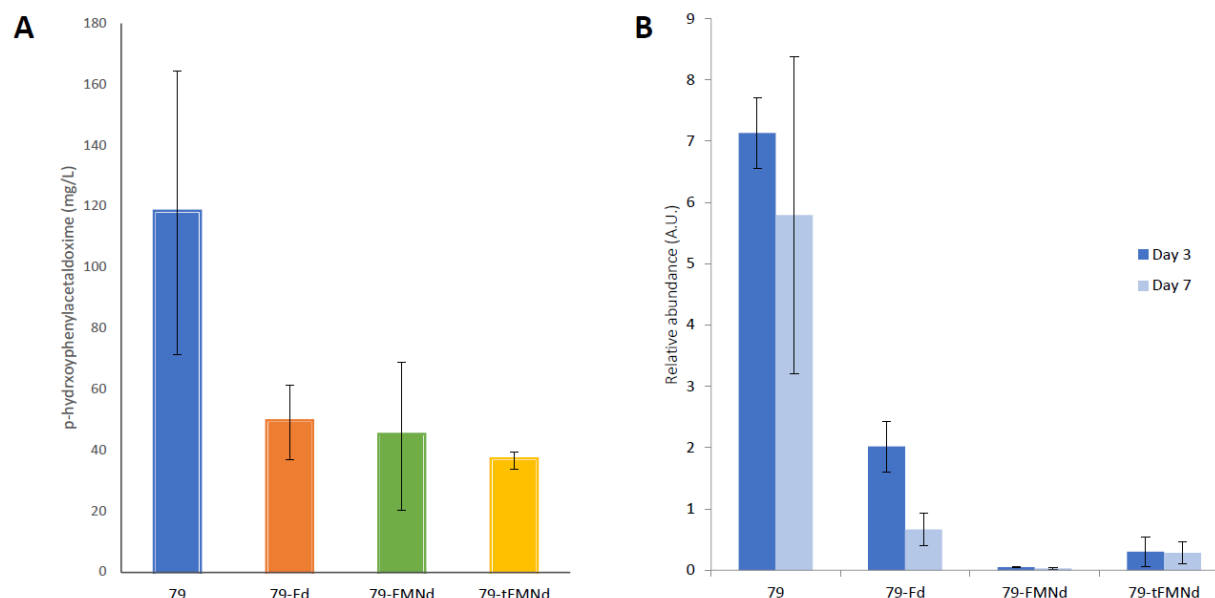
Figure 5. In vivo oxime yield and enzyme abundance. (A) Absolute p -hydroxyphenylacetaldoxime levels were measured by LC-MS at the end of a 7-day fermentation. (B) Relative protein abundance levels were measured on day 3 and day 7 of the fermentation.
