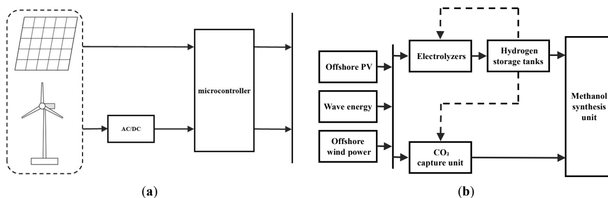
Figure 1. Representative research outcomes: (a) Structure of wind-PV power-generation system; (b) Full-coupling framework of electricity-hydrogen-carbon-methanol.
