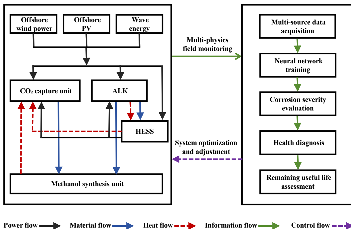
Figure 3. Whole-chain Collaborative Optimization System for Offshore Renewable Energy Hydrogen Production.
