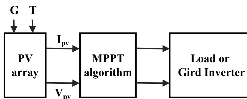
Figure 2. Topology of the maximum-power-point tracking system.
