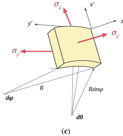
Figure 3. Conceptual model for high-Reynolds-number laminar flow. (a) No-slip pipe-flow at hypothesized transition condition, where virtual-shell curvature radius equals physical pipe radius R_S = R . A high-Reynolds number laminar flow inside a smaller radius pipe R_1 \leq R = R_S can be conceptualized as a sub-region of this full-scale reference pipe. (b) Wall shear stress \tau constitutes a directional component of critical-tensile-force flow \gamma_v : \tau = \gamma_v \sin \varphi . When \varphi = 90^\circ , wall shear stress at transition R = R_S equals \tau_{w,c} = \gamma_v . (c) Micro-element within local x'y'z' coordinate system, where \sigma_{x'} , \sigma_{y'} are related to \gamma_v , respectively, and \sigma_{z'} = p(z) .
