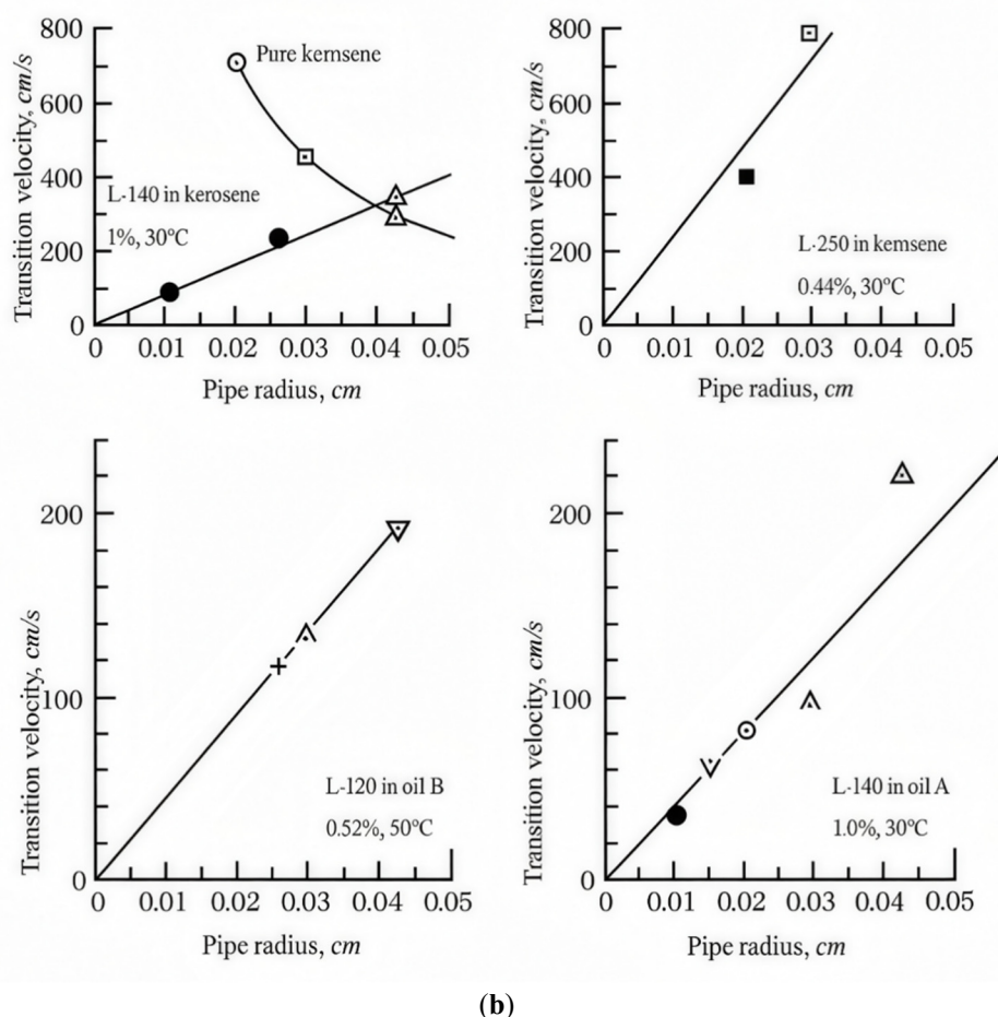
Figure 2. The relationship between the transition velocity of laminar flow and the radius of the pipe. (a) Schematic diagram contrasting transition velocity versus pipe radius for two cases. Red circles: trend derived from the present critical-tensile-force-flow criterion; black squares: trend inferred from classical critical-Reynolds-number criterion. These points are theoretical schematic sampling points, not experimental measurements. Figure 2a is a conceptual schematic diagram without quantitative axis scales. Two curves partition the parameter space into four zones I–IV. Zone I: laminar flow; Zone II: turbulent flow; Zone III: predicted laminar according to critical-Reynolds-number criterion but observed as early turbulence in experiments [10]; Zone IV: predicted turbulent by critical-Reynolds-number criterion but achievable as laminar via active wall suction [16]. (b) Reproduced experimental early-turbulence data for different polymer-solution systems; transition velocity scales linearly with pipe radius and extrapolates toward the origin, consistent with critical-shear-stress-controlled structural-turbulence onset reported in literature [10].
