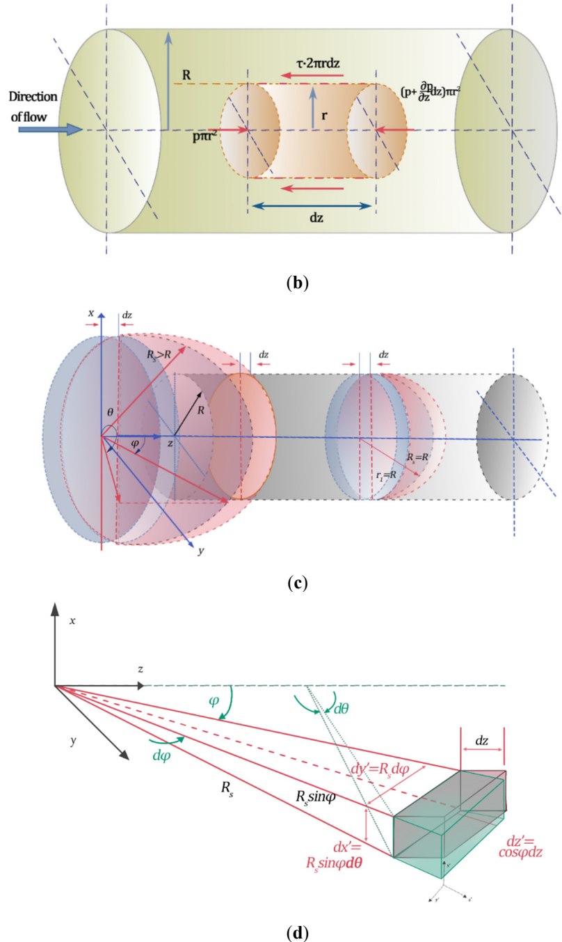
Figure 1. Laminar spherical fluid layers in a pipe and the microelement for force analysis. (a) A spherical shell under a load q uniformly distributed over the planform [21]. The distributions of the membrane force flow N_{\varphi\varphi} and N_{\theta\theta} are given as: N_{\varphi\varphi} = -\frac{qR}{2} , N_{\theta\theta} = -\frac{qR\cos 2\varphi}{2} . (b) Steady laminar and incompressible flow through pipe [22]. The flow direction is defined as the z -direction. Laminar-flow conditions: u_r = u_\theta = 0 , u_z(r) = u_0 \left(1 - \frac{r^2}{R^2}\right) , u_0 = -\frac{R^2}{4\mu} \frac{\partial p}{\partial z} , with \frac{\partial p}{\partial z} < 0 . Wall shear stress at r = R : \tau_w = \mu \left. \frac{du}{dr} \right|_{r=R} = -\frac{2\mu u_0}{R} . (c) Spherical-shell-shaped fluid layers with stream-wise thickness dz . R_s denotes the single curvature radius of the virtual layer, R_s \geq R , subscript S denotes “spherical”. (d) A differential element of a spherical shell in local x'y'z' coordinates, where dz' = \cos\varphi dz , dx' = r d\theta = R_s \sin\varphi d\theta , dy' = R_s d\varphi . Force flows in the x' - and y' -coordinates correspond to \gamma_{\theta\theta} and \gamma_{\varphi\varphi} respectively, pressure in the z' -direction equals \sigma_{z'} = p(z) .
