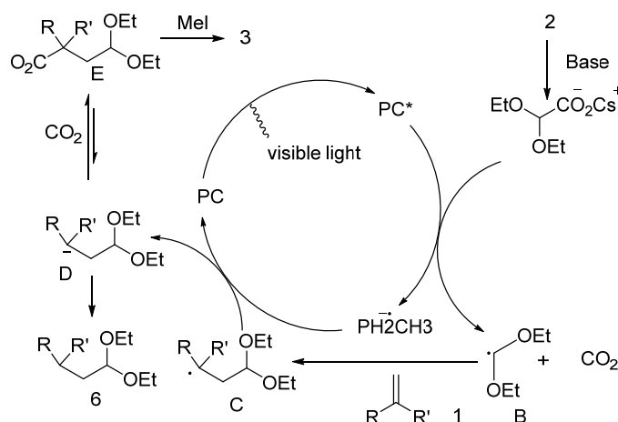
Scheme 13. Plausible reaction mechanism.
