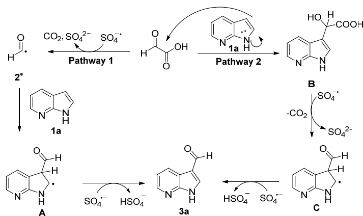
Scheme 10. Plausible reaction mechanism.
