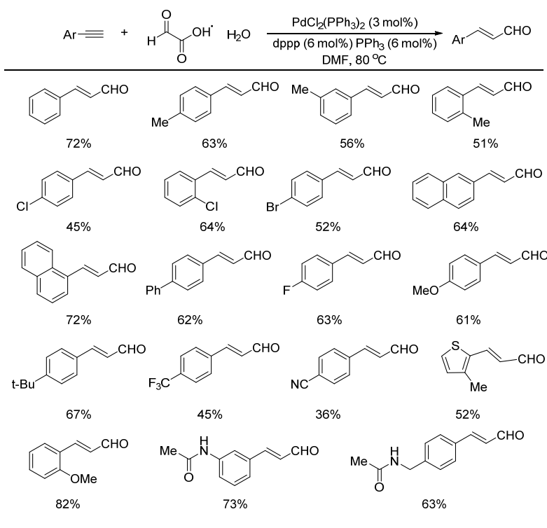
Figure 5. Palladium-catalyzed hydroformylation of terminal arylacetylenes with glyoxylic acid.
