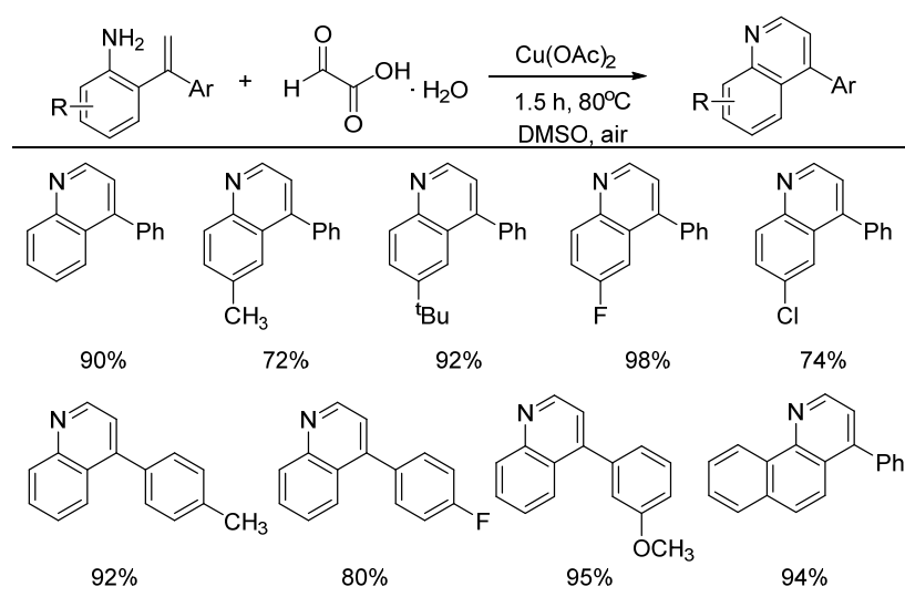
Figure 21. Copper-mediated [5+1] annulation of 2-vinylanilines and glyoxylic acid.
