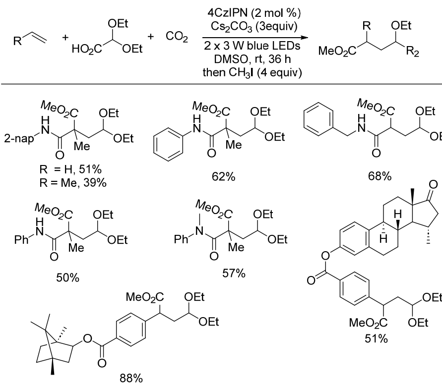
Figure 13. Visible-light-induced photoredox catalytic formylation involving glyoxylic acid.
