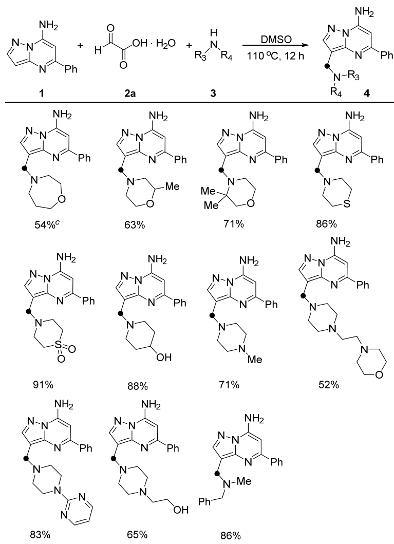
Figure 25. Synthesis of C3-aminomethylated pyrazolo [1,5-a] pyrimidines.
