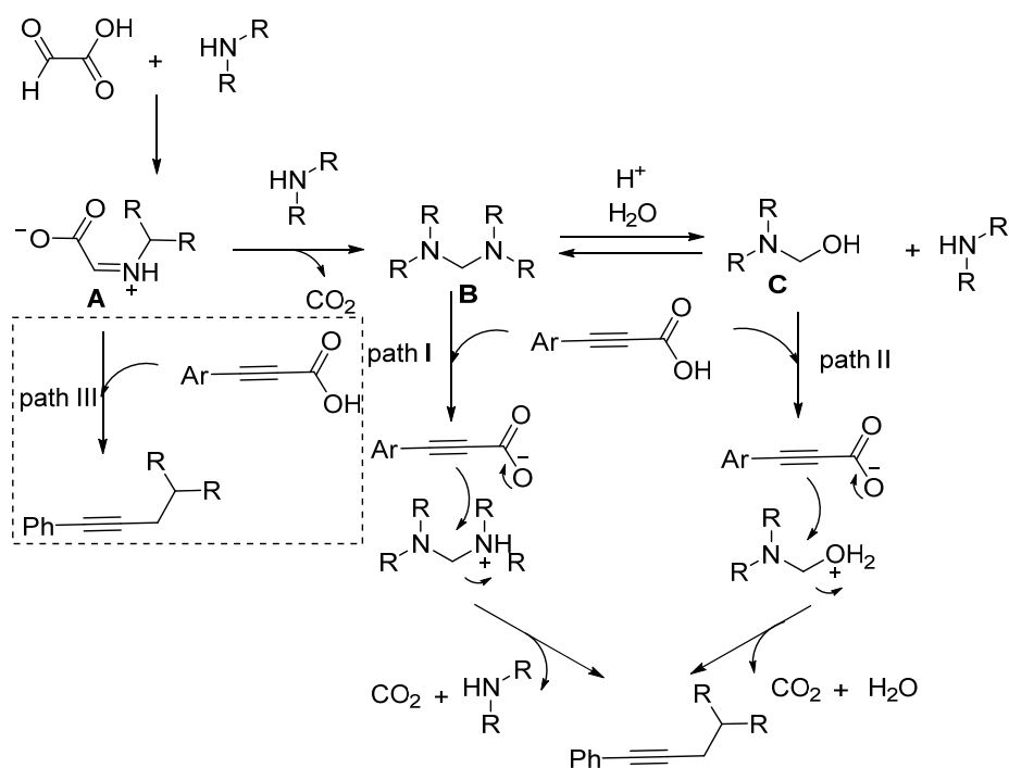
Scheme 20. Plausible reaction mechanism.
