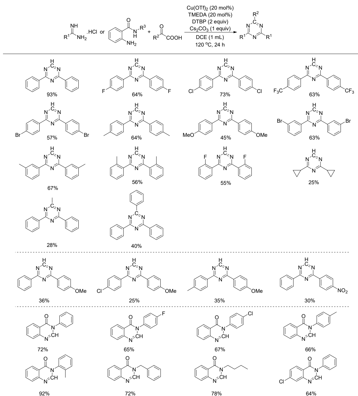
Figure 18. Copper-catalyzed oxidative decarboxylative amination of glyoxylic acid with dinucleophilic amines.
