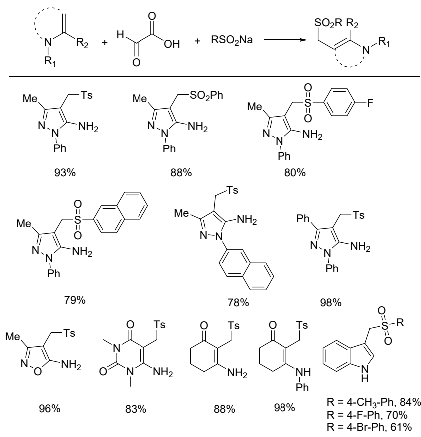
Figure 23. C4-sulfonylmethylation of pyrazol-5-amines with glyoxylic acid and sodium sulfinates.
