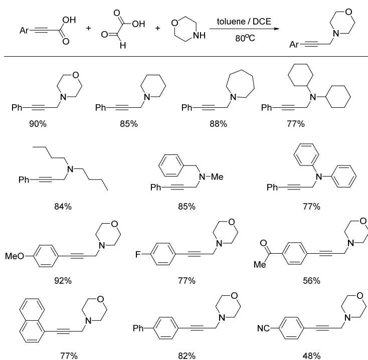
Figure 20. Three-component reaction of glyoxylic acid, arylalkynoic acids, and amines.
