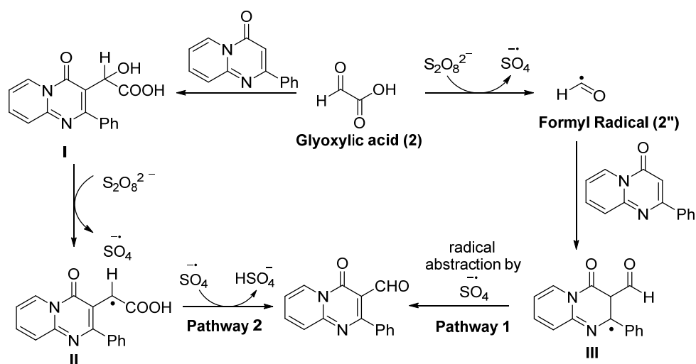
Scheme 15. Plausible reaction mechanism (formylation pathway).
