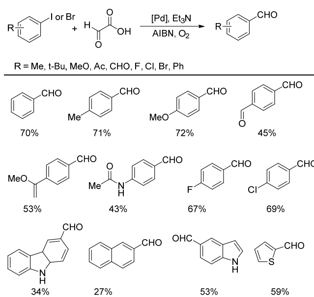
Figure 7. Palladium-catalyzed formylation of aryl halides with glyoxylic acid.
