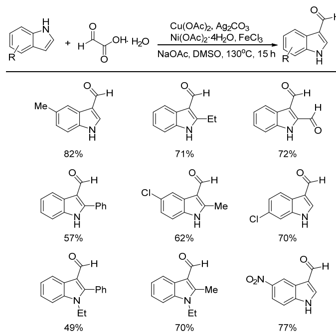
Figure 4. Four-metal-salt catalyzed formylation of indoles with glyoxylic acid.
