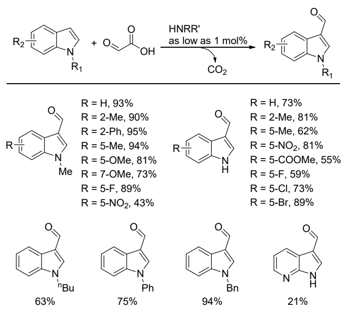
Figure 6. Amine-catalyzed electrochemical formylation of indoles with glyoxylic acid.
