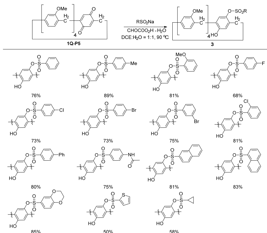
Figure 36. Reductive addition to pillararene-quinone.
