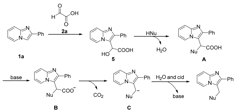
Scheme 24. Plausible reaction mechanism.
