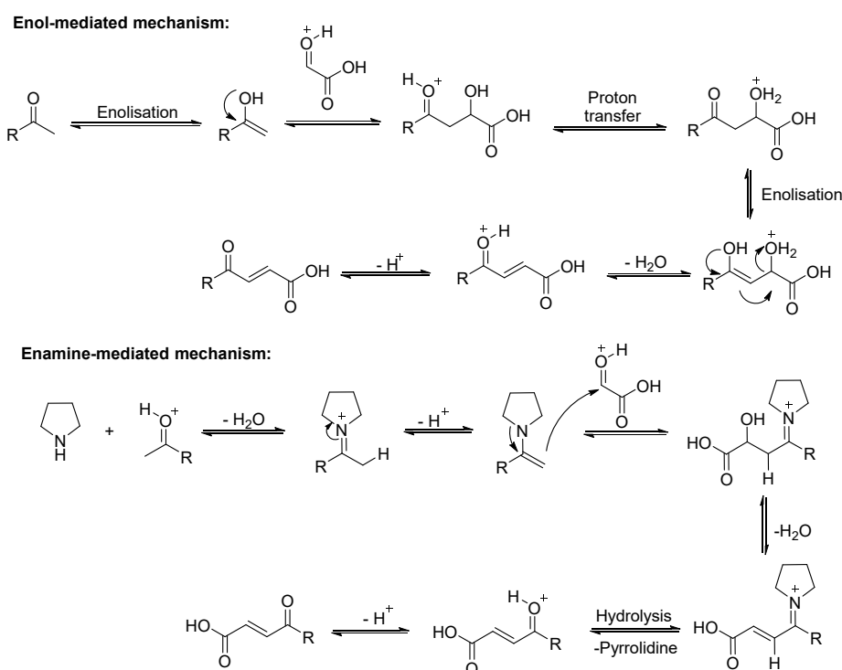
Scheme 28. Plausible reaction mechanism.
