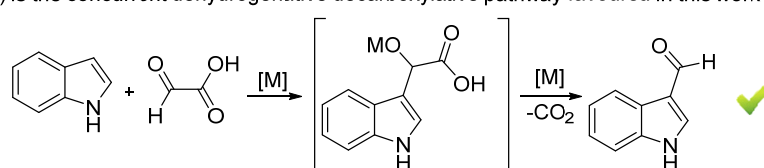
Scheme 4. Plausible reaction mechanism.
