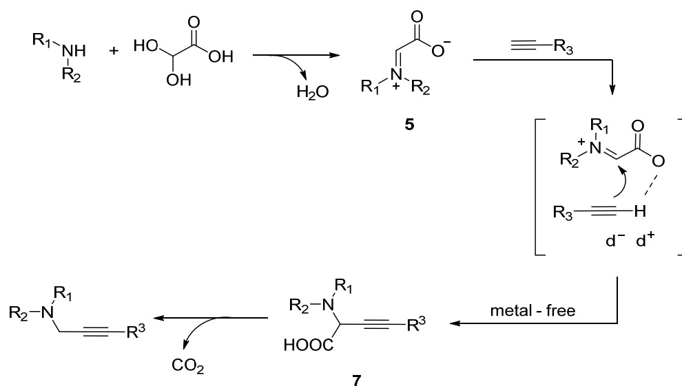
Scheme 19. Plausible reaction mechanism.
