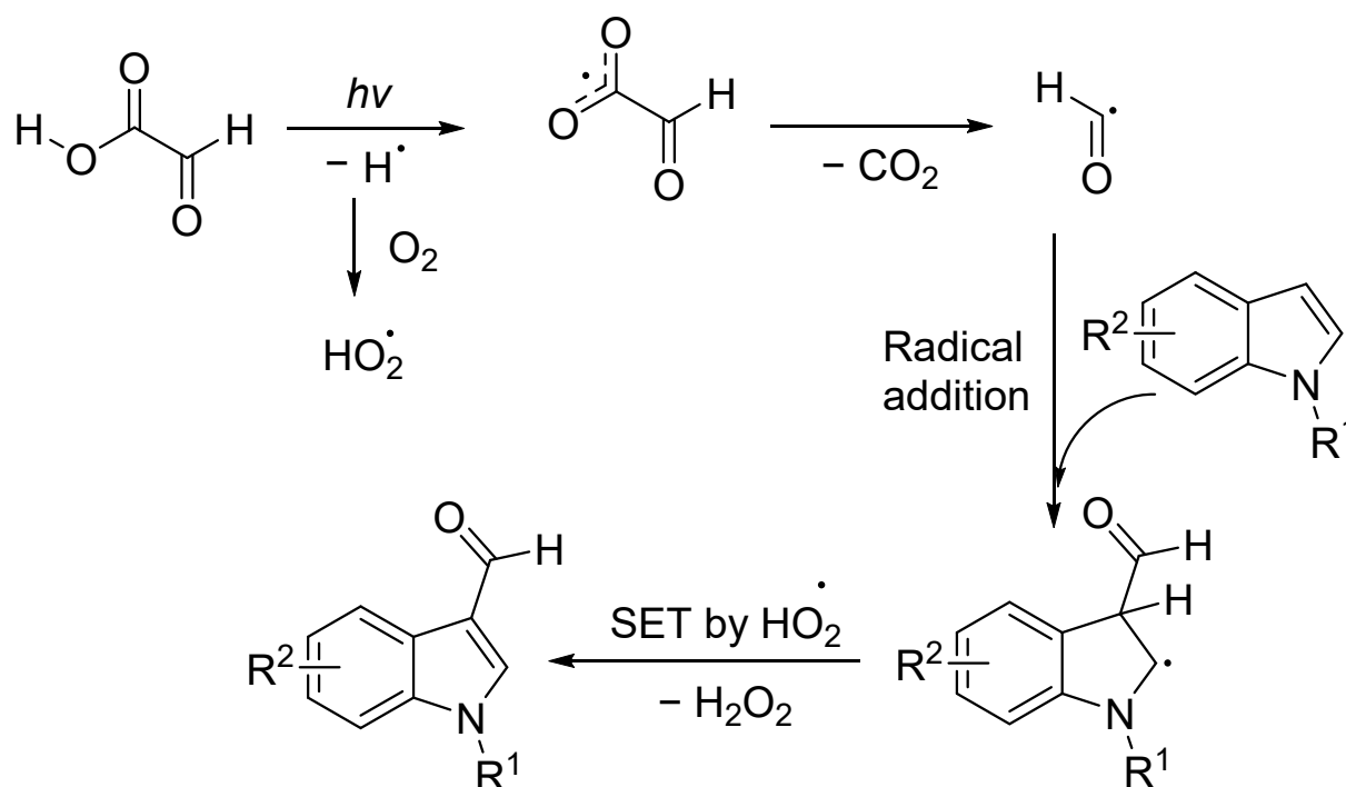
Scheme 12. Plausible reaction mechanism.
