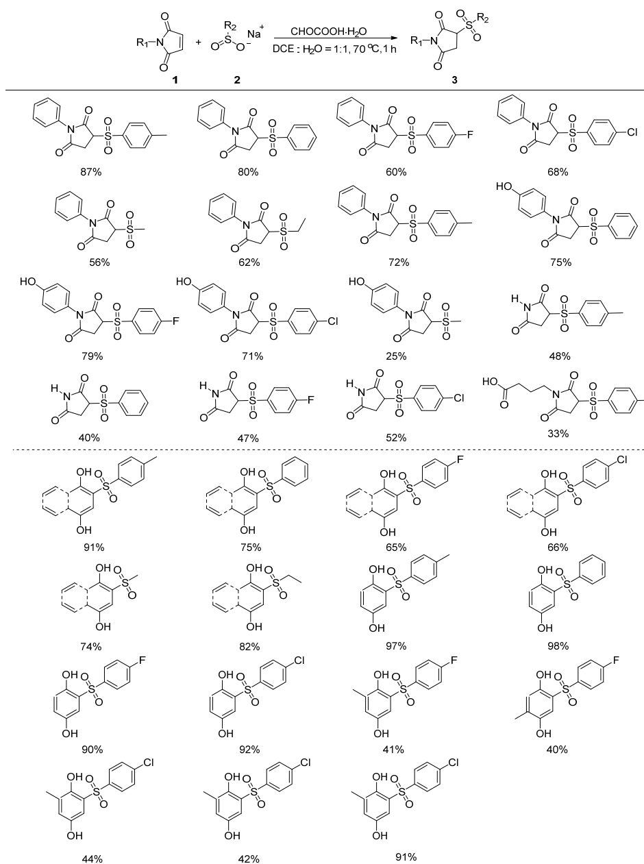
Figure 35. \alpha -sulfonylation of maleimides.
