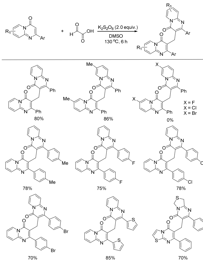
Figure 16. Glyoxylic acid as a methylene source.
