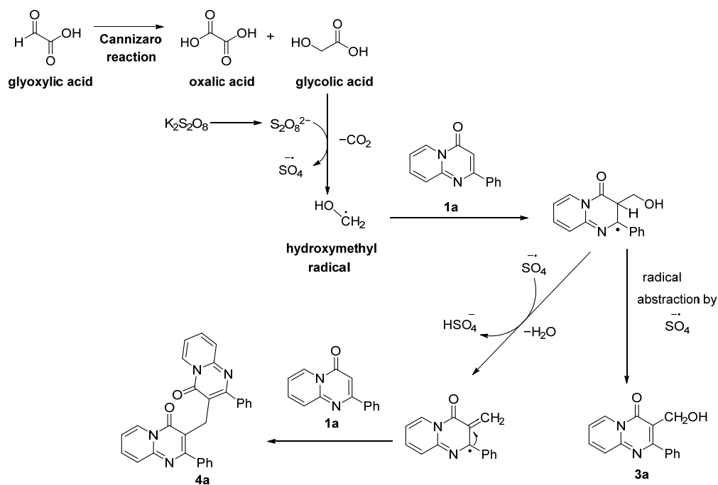
Scheme 16. Plausible reaction mechanism (methylenation pathway).
