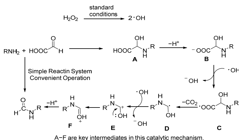
Scheme 11. Plausible reaction mechanism.
