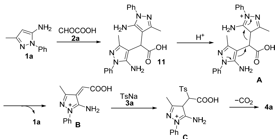
Scheme 23. Plausible reaction mechanism.
