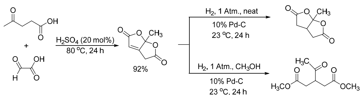
Figure 26. Condensation-cyclization of levulinic acid with glyoxylic acid.
