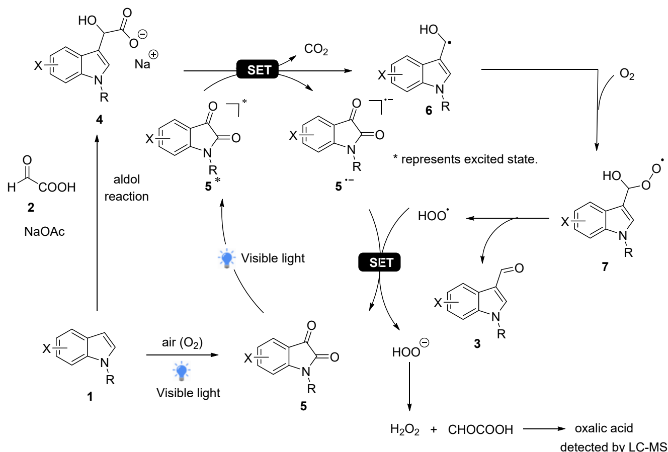
Scheme 8. Plausible reaction mechanism.
