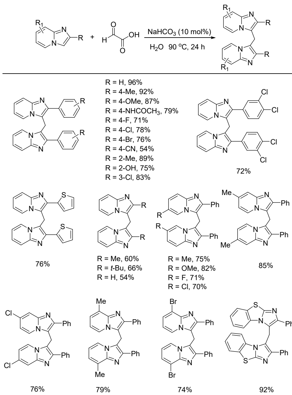
Figure 24. Methylenation of imidazo[1,2- a ]pyridines.
