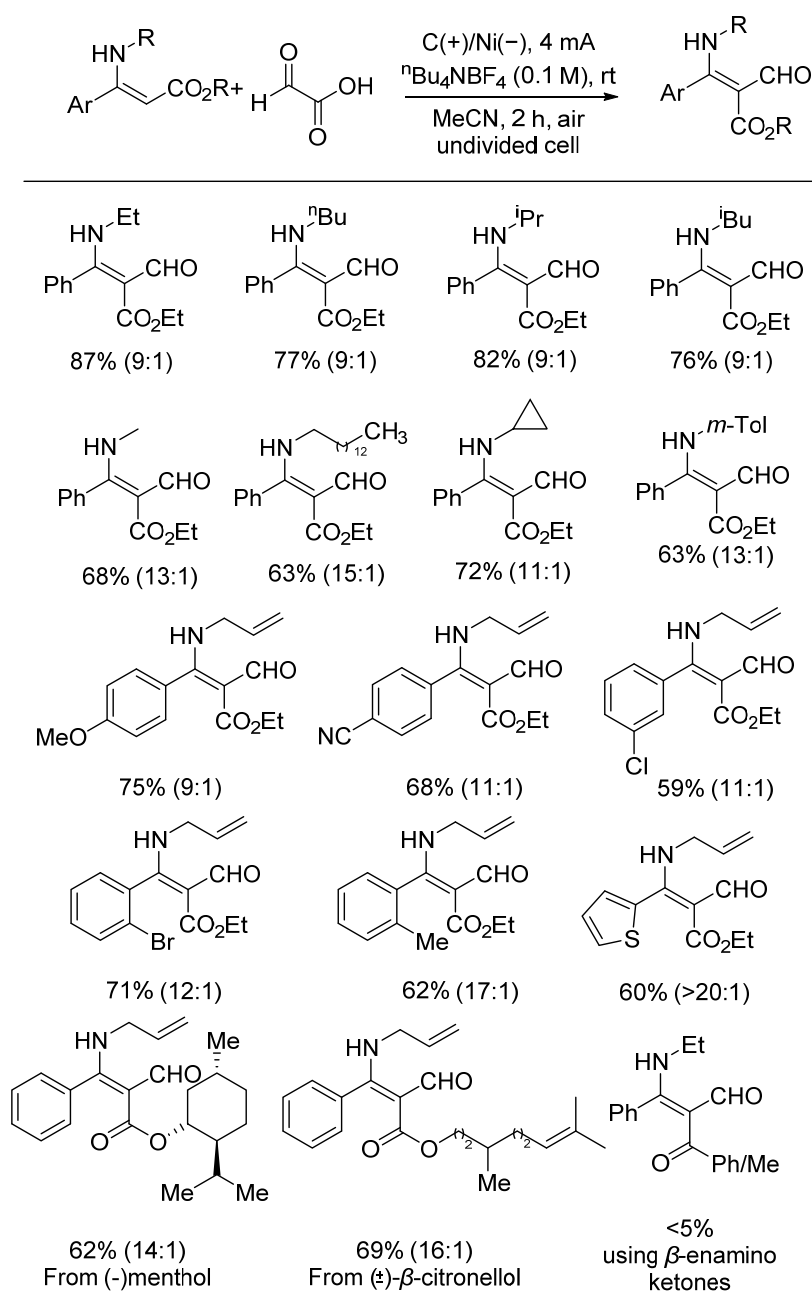
Figure 14. Electrochemically driven formylation using glyoxylic acid.
