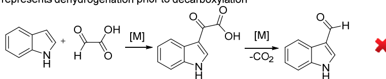
Figure 4. Four-metal-salt catalyzed formylation of indoles with glyoxylic acid.
