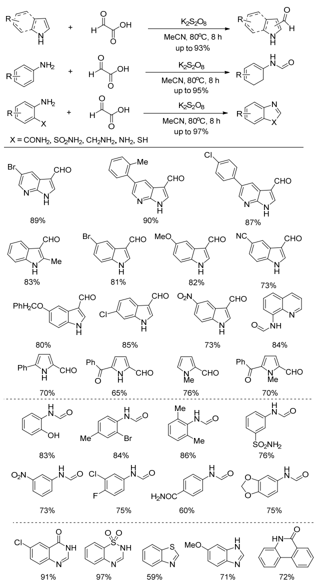
Figure 10. K 2 S 2 O 8 -catalyzed formylation of N -heteroarenes and anilines.
