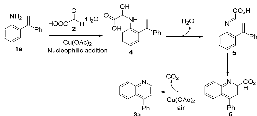
Scheme 21. Plausible reaction mechanism.
