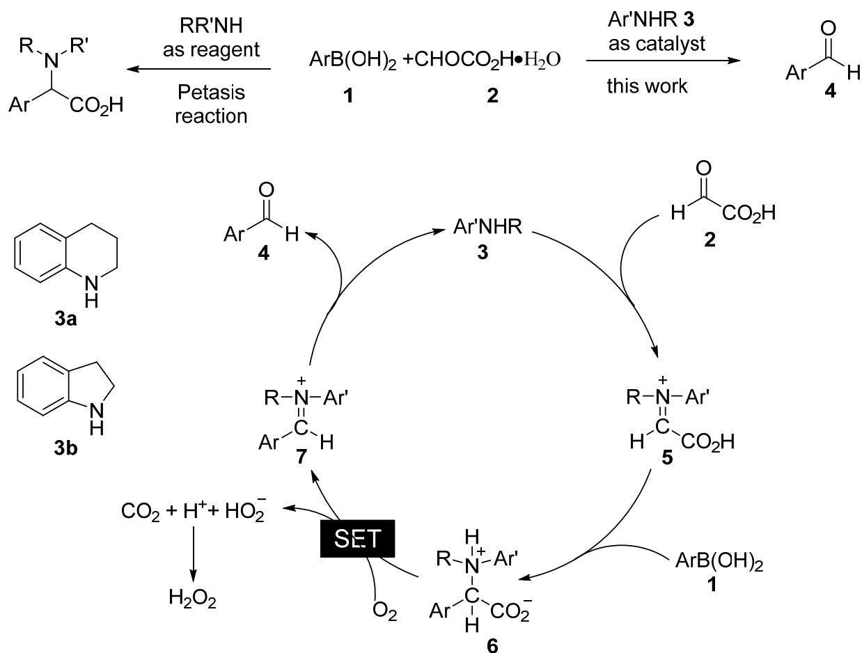
Scheme 1. Plausible reaction mechanism.
