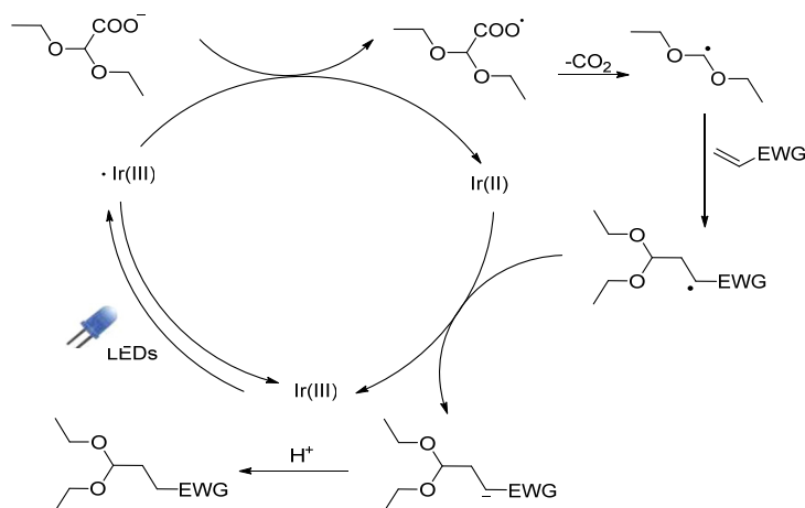
Scheme 27. Plausible reaction mechanism.
