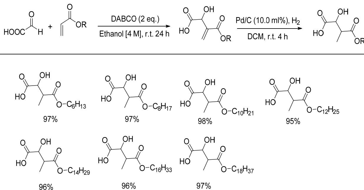
Figure 31. Synthesis of novel amphiphilic compounds using glyoxylic acid.
