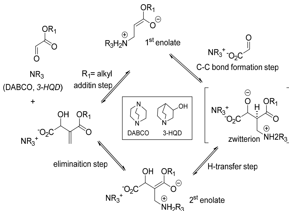
Scheme 30. Plausible reaction mechanism.
