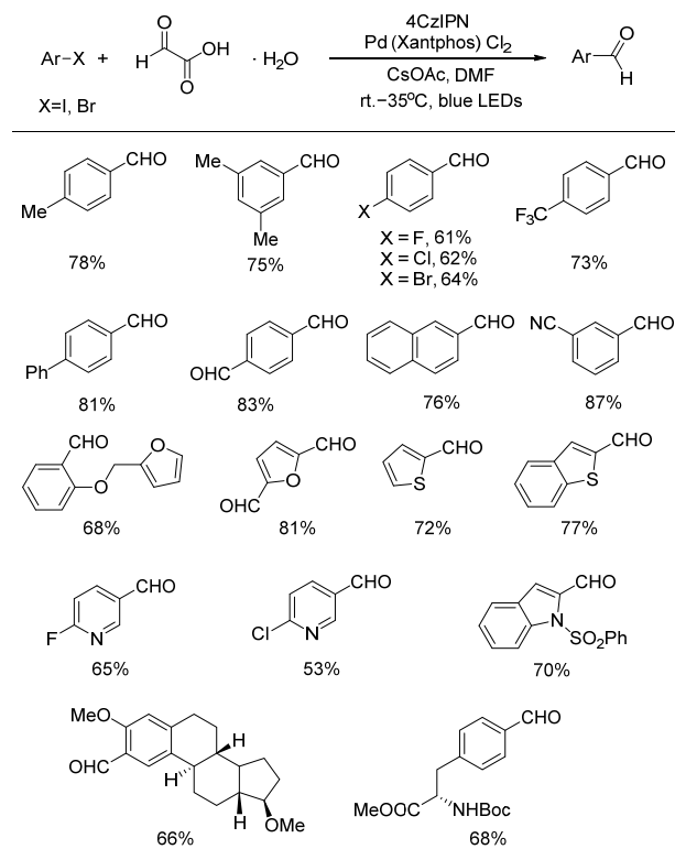
Figure 3. Palladium-catalyzed formylation of aryl halides with glyoxylic acid.
