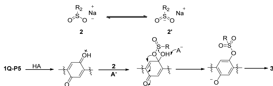
Scheme 34. Plausible reaction mechanism.
