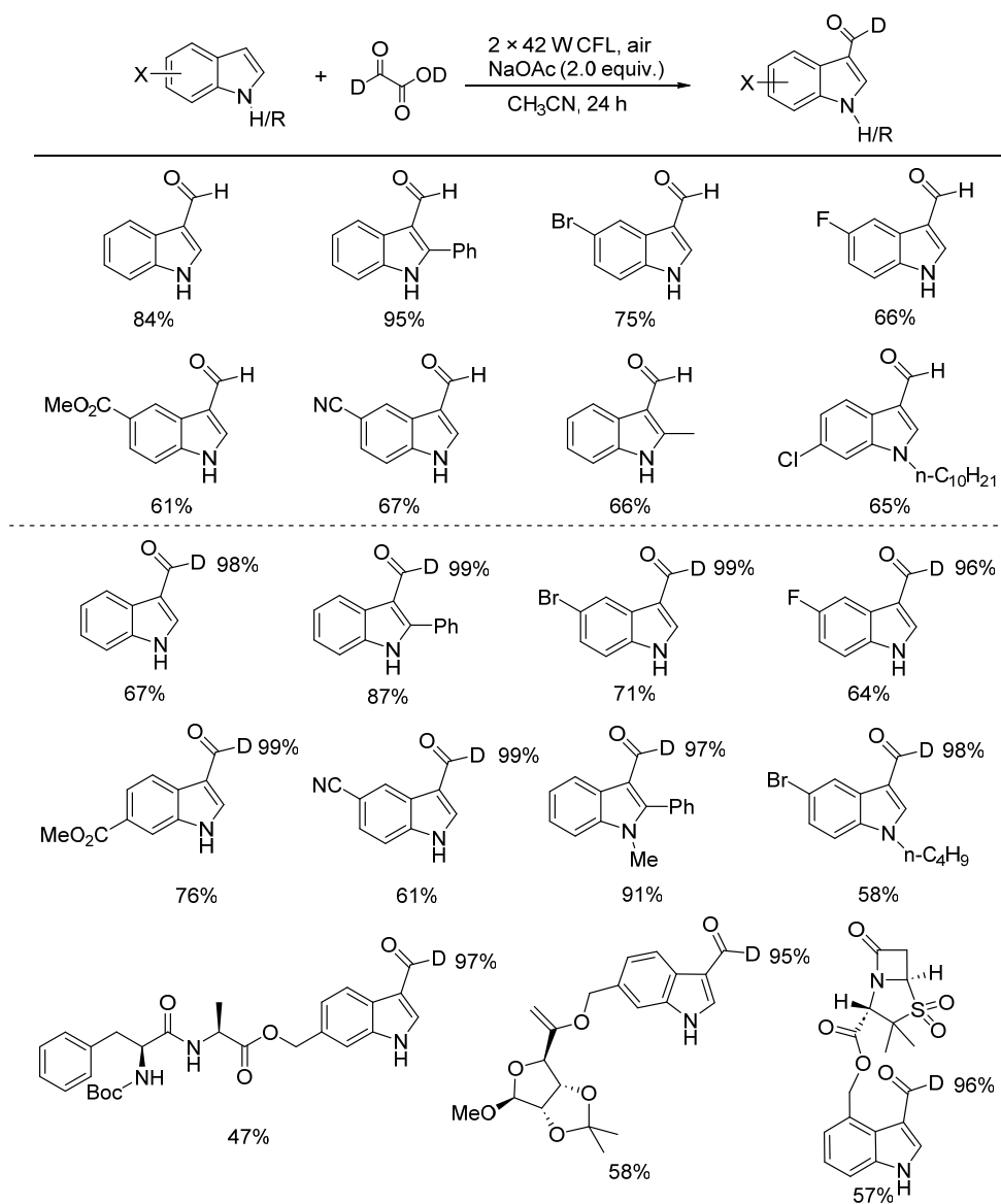
Figure 8. Amine-catalyzed formylation of indoles with deuterated glyoxylic acid.
