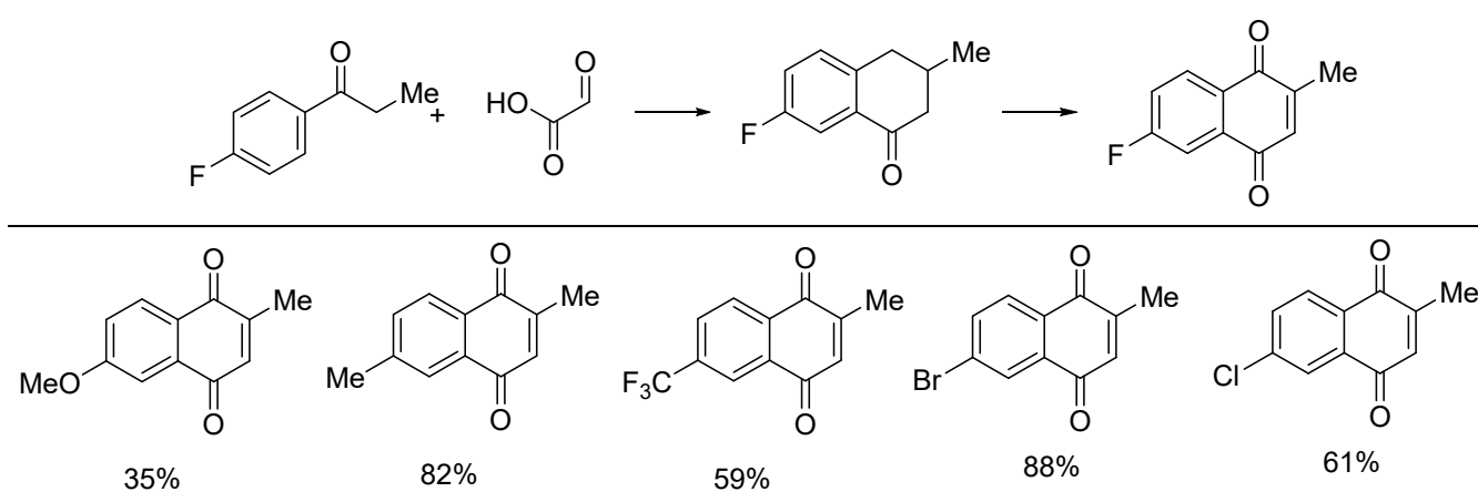
Figure 29. Condensation-cyclization of arylpropiophenones with glyoxylic acid.
