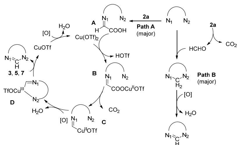
Scheme 18. Plausible reaction mechanism.
