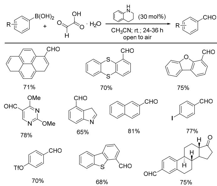
Figure 1. Tetrahydroquinoline-catalyzed formylation of arylboronic acids with glyoxylic acid.
