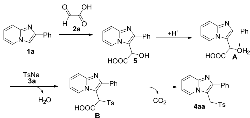
Scheme 22. Plausible reaction mechanism.
