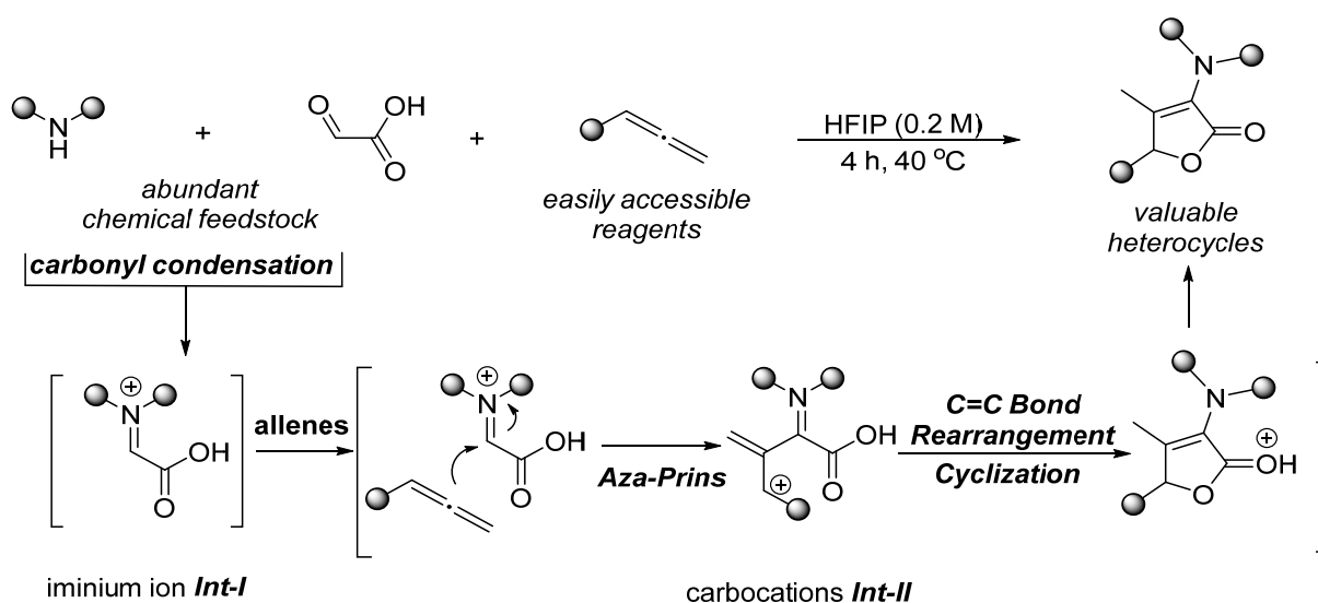
Scheme 32. Plausible reaction mechanism.
