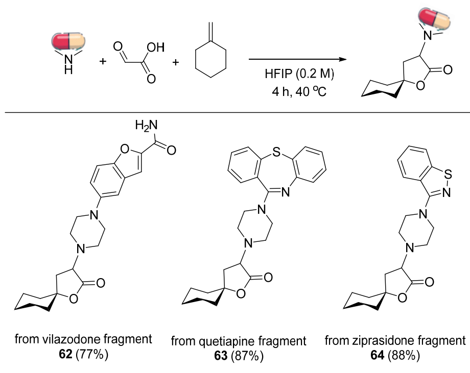
Figure 33. Late-Stage Functionalization of Pharmacophore.
