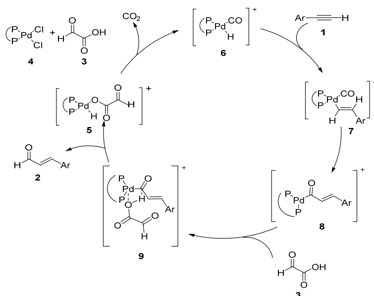
Scheme 5. Plausible reaction mechanism.
