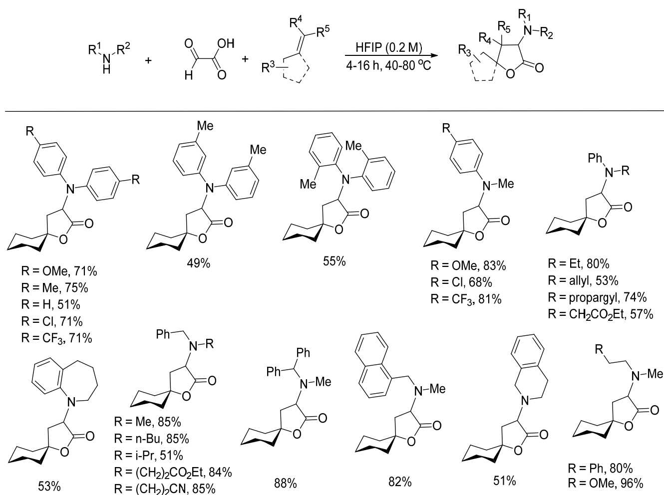
Figure 32. Reactivity of various secondary amines with glyoxylic acid and methylenecyclohexane.
