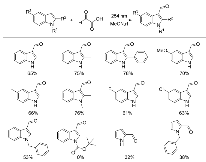
Figure 12. Synthesis of indole-3-carboxaldehyde derivatives.
