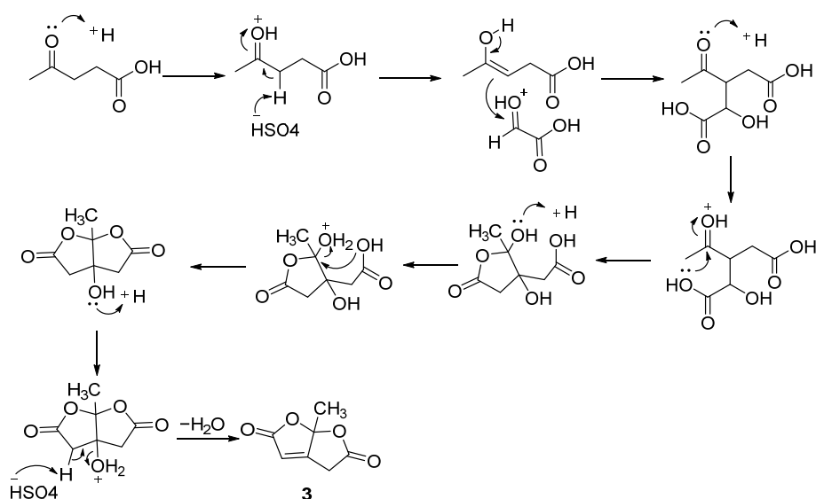
Scheme 26. Plausible reaction mechanism.
