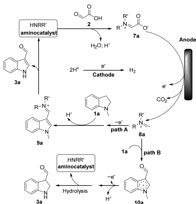
Scheme 6. Plausible reaction mechanism.
