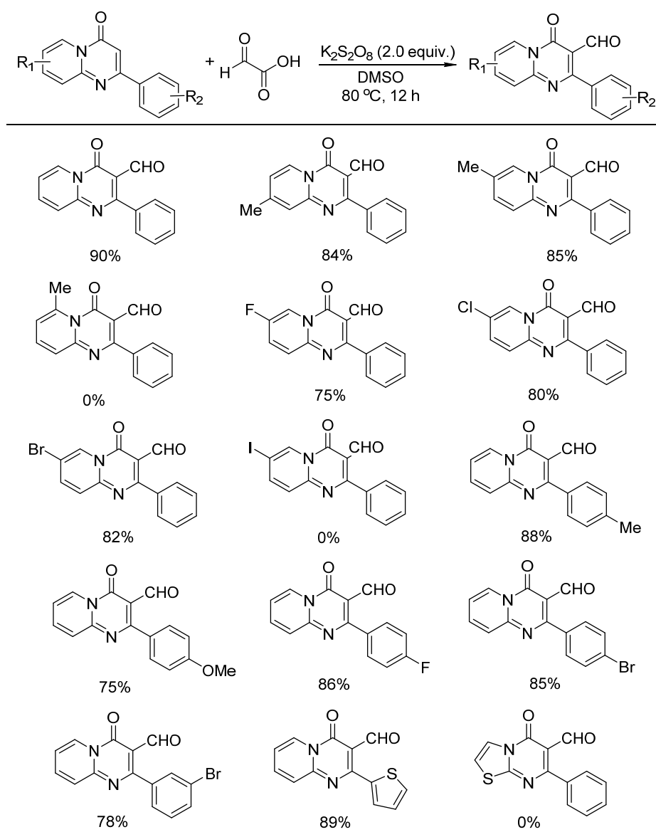
Figure 15. Glyoxylic acid as a hydroxymethyl source.
