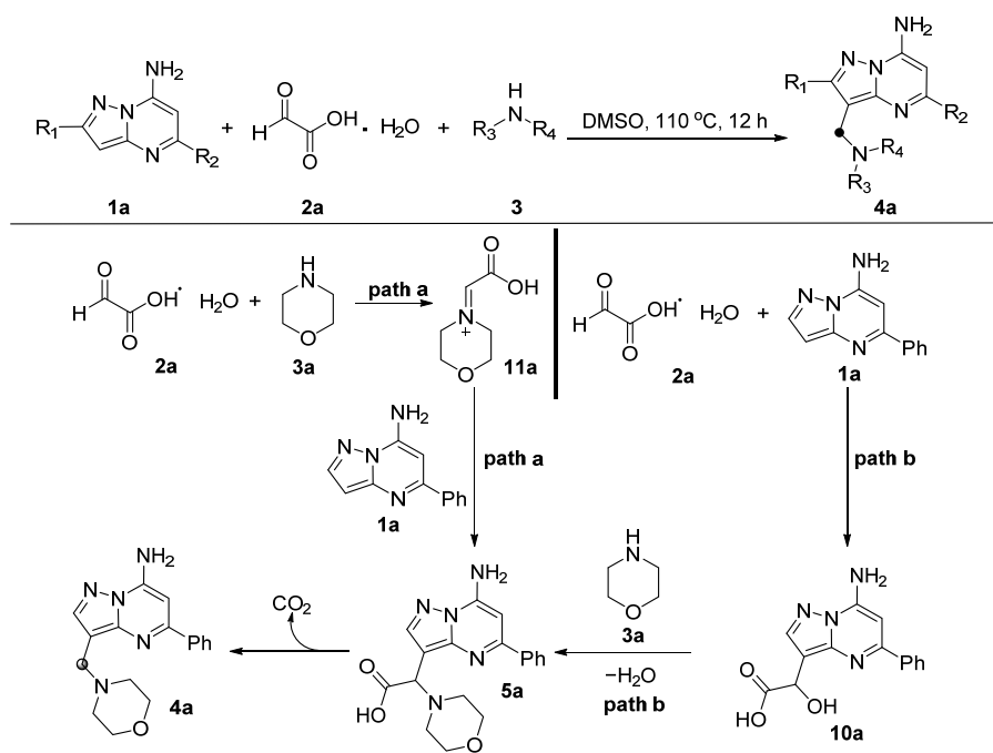
Scheme 25. Plausible reaction mechanism.
