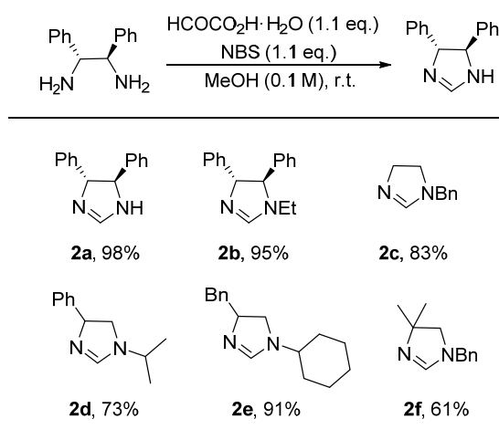
Figure 17. Synthesis of 2-H-imidazoline derivatives.
