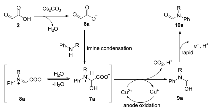
Scheme 2. Plausible reaction mechanism.
