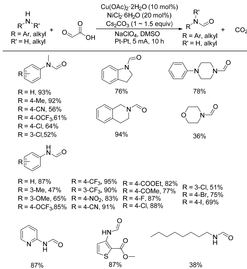
Figure 2. Glyoxylic-acid-involved N -formylation.
