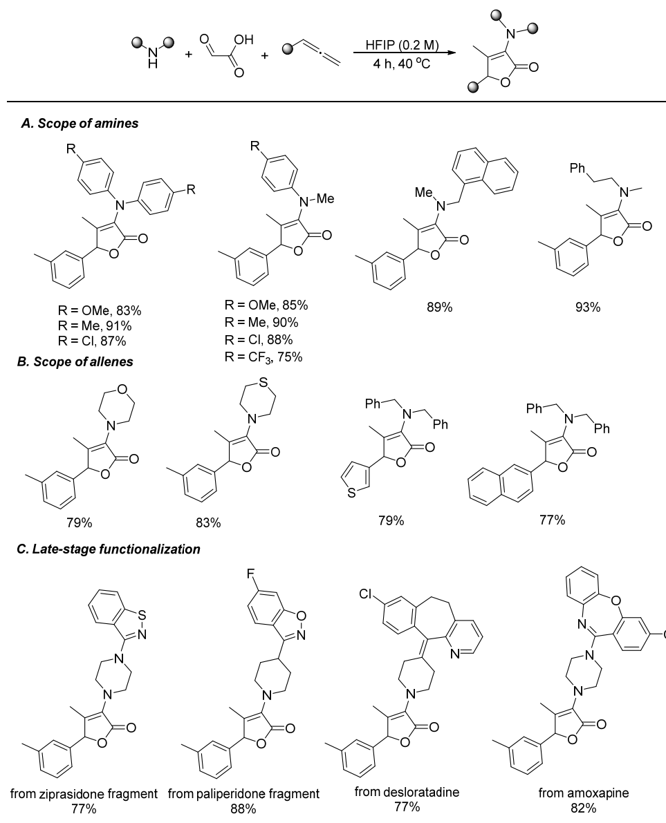
Figure 34. Scope of the hydroaminoalkylation-aza-Prins reaction.
