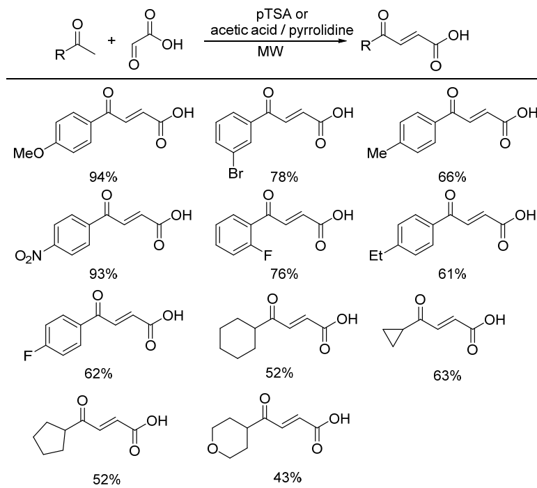
Figure 28. Microwave-assisted aldol condensation of methyl ketones with glyoxylic acid.
