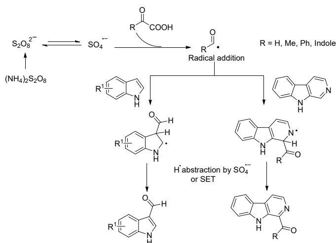
Scheme 9. Plausible reaction mechanism.
