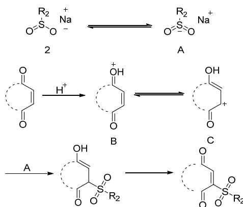
Scheme 33. Plausible reaction mechanism.
