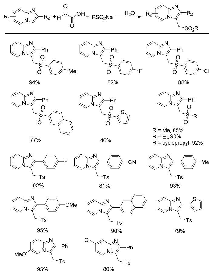
Figure 22. C3-sulfonylmethylation of imidazo[1,2- a ]pyridines with glyoxylic acid and sodium sulfinates.
