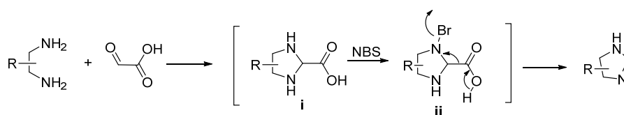
Scheme 17. Plausible reaction mechanism.
