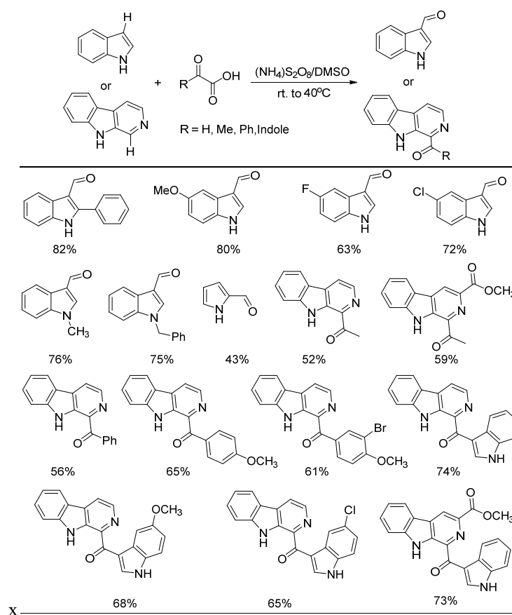
Figure 9. Ammonium persulfate-mediated formylation of indoles or \beta -carbolines with glyoxylic acid.
