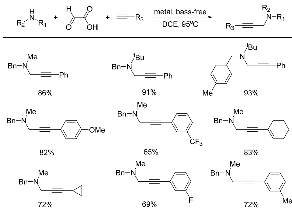
Figure 19. Three-component reaction of glyoxylic acid, secondary amines, and alkynes.
