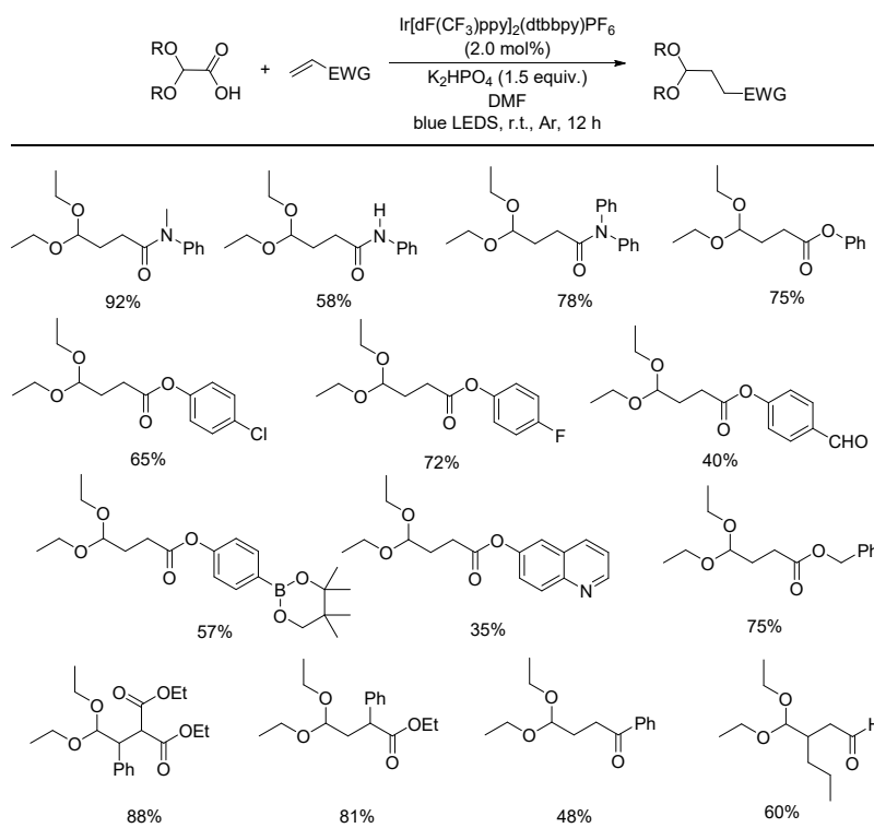
Figure 27. Iridium photoredox-catalyzed decarboxylative Michael addition of glyoxylic acid acetal.
