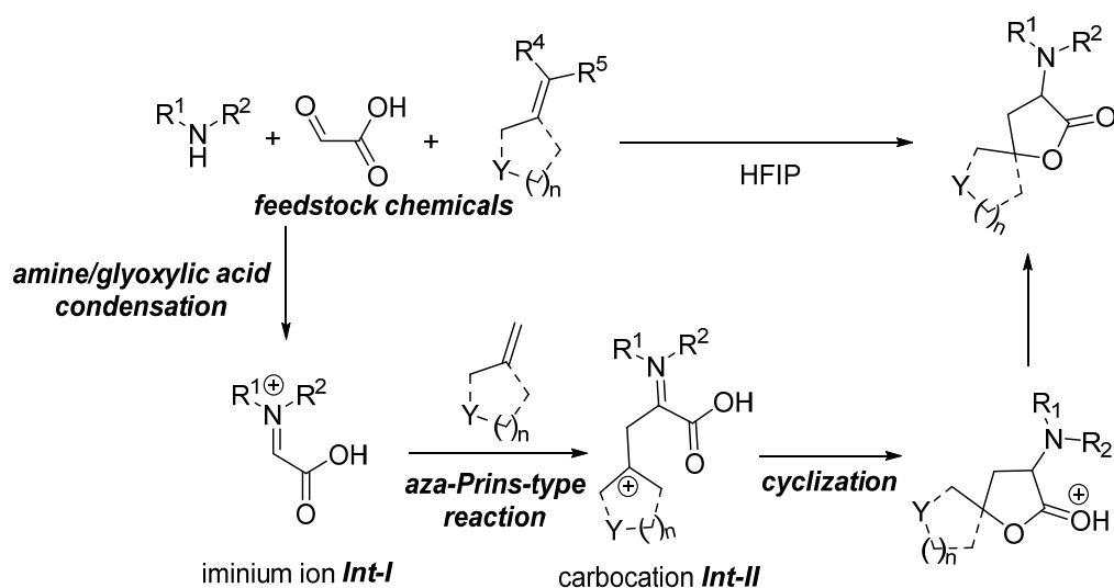
Scheme 31. Plausible reaction mechanism.
