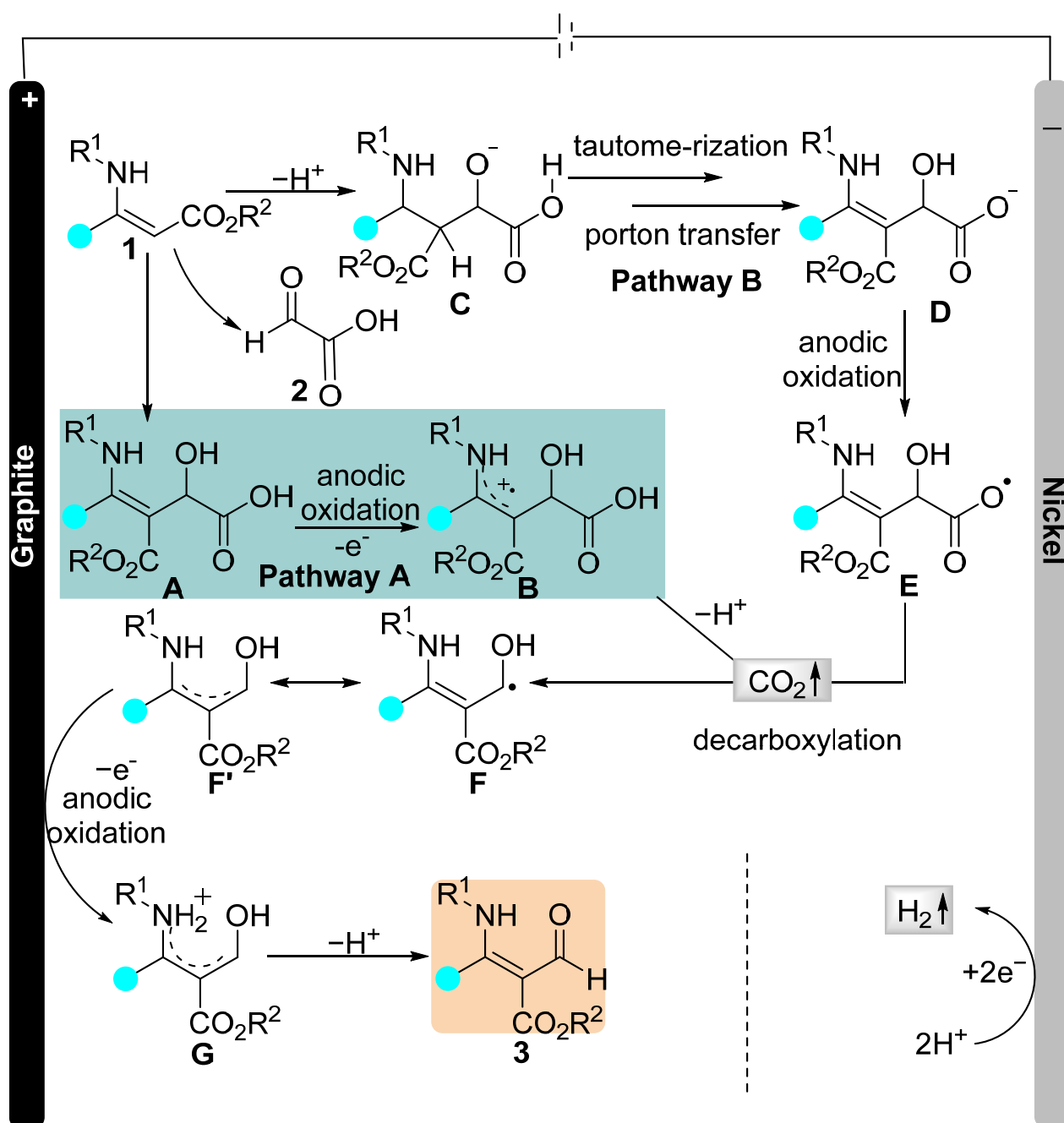
Scheme 14. Plausible reaction mechanism.
