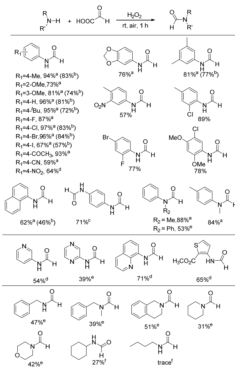
Figure 11. Synthesis of formamides. a Reaction conditions: 1 (0.3 mmol), 2a (0.3 mmol, 50% in water), \text{H}_2\text{O}_2 (2.0 equiv, 30% in water), DMSO (1.5 mL), at rt under air for 1 h. Yields shown are of isolated products. b \text{H}_2\text{O} as the solvent. c 0.6 mmol of 2a . d 60 °C for 3 h. e 90 °C for 6 h. f 120 °C for 6 h.
